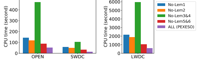
Fig. 8: Ablation study (OPEN, SWDC, and LWDC).
