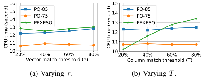
Fig. 7: Comparison to approximate method PQ (SWDC).
