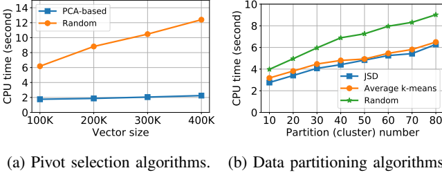
Fig. 6: Pivot selection and data partitioning (LWDC).
